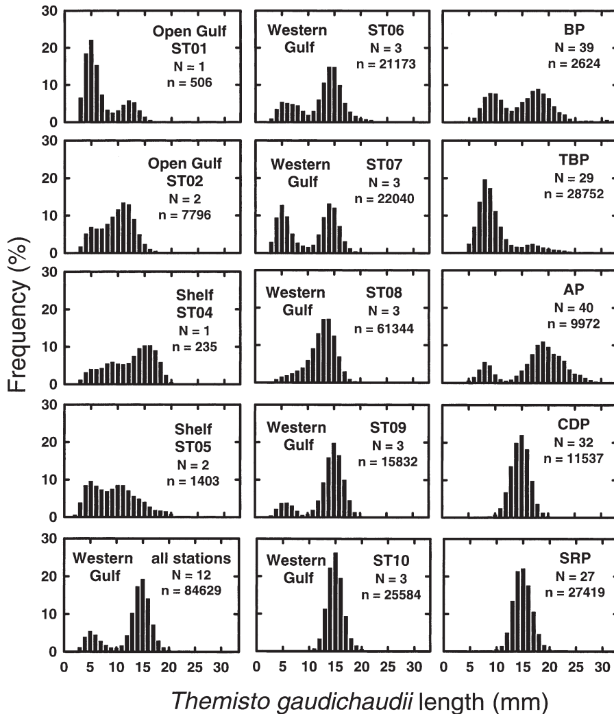
Fig. 2. Themisto gaudichaudii . Length-frequency distribution in net hauls and in the diet of seabirds. Western gulf stations: pooled results from Stns 6, 7, 9 and 10; BP: blue petrel; TBP: thin-billed prion; AP: Antarctic prion; CDP: common diving petrel; SRP: southern rockhopper penguin. N: number of net hauls or food samples; n: number of individuals
