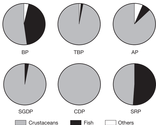
Fig. 3. Themisto gaudichaudii . Composition by fresh mass of the diet of seabirds in the 1996 summer months. BP: blue petrel; TBP: thin-billed prion; AP: Antarctic prion; SGDP: South Georgian diving petrel; CDP: common diving petrel; SRP: southern rockhopper penguin
