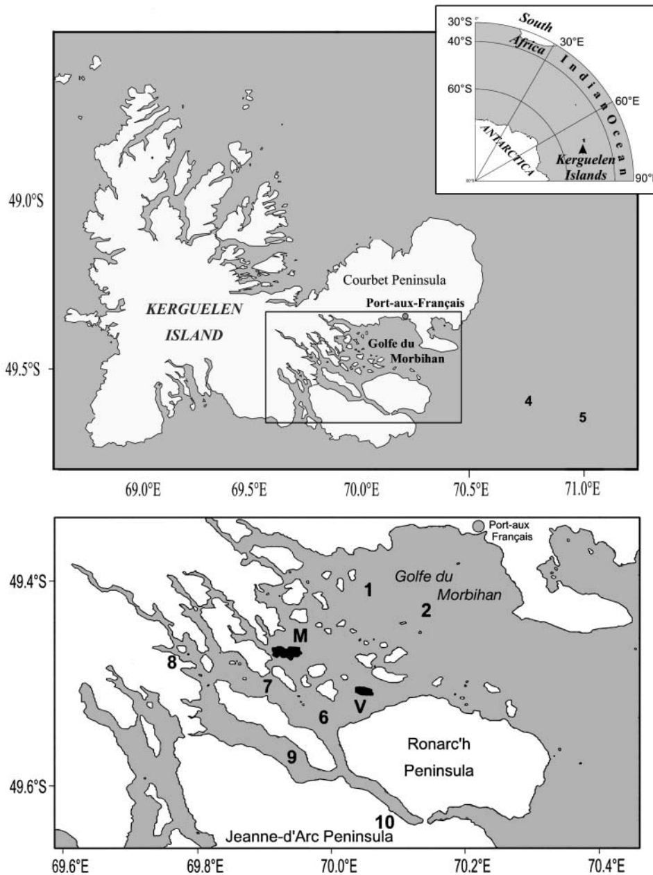
Fig. 1. Themisto gaudichaudii . Map of Kerguelen Islands (upper panel) and details of the eastern part of the archipelago (lower panel). Numbers 1 to 10: locations of macrozooplanktonic stations (note that there is no Station 3), M: Ile Mayes; V: Ile Verte
