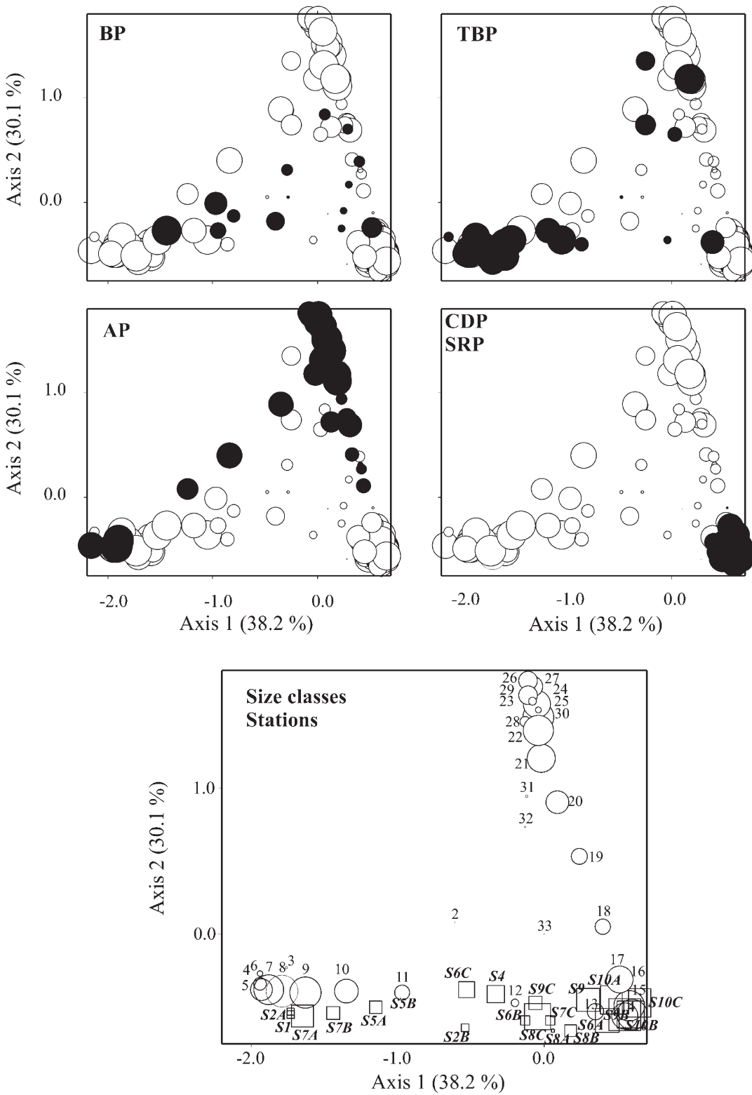
Fig. 4. Themisto gaudichaudii . Plan of the axes 1 and 2 of the correspondence analysis of the size classes in the diet of seabirds (4 upper panels) and net hauls (lower panel). Bird species, net hauls and size classes are presented in different graphics to avoid overloading the representation, but the space is identical. The symbol for each object is proportional to its relative contribution, an index of the quality of the representation. BP: blue petrel; TBP: thin-billed prion; AP: Antarctic prion; CDP: common diving petrel; SRP: southern rockhopper penguin; N: number of net hauls or food samples; n: number of individuals
